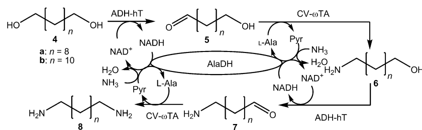
Scheme 2. Double bioamination of long-chain n -alkane-1, \omega -diols.
